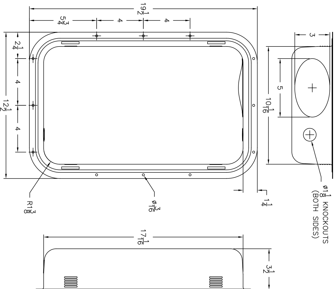
DBX1000M BOX DIMENSION VIEW
